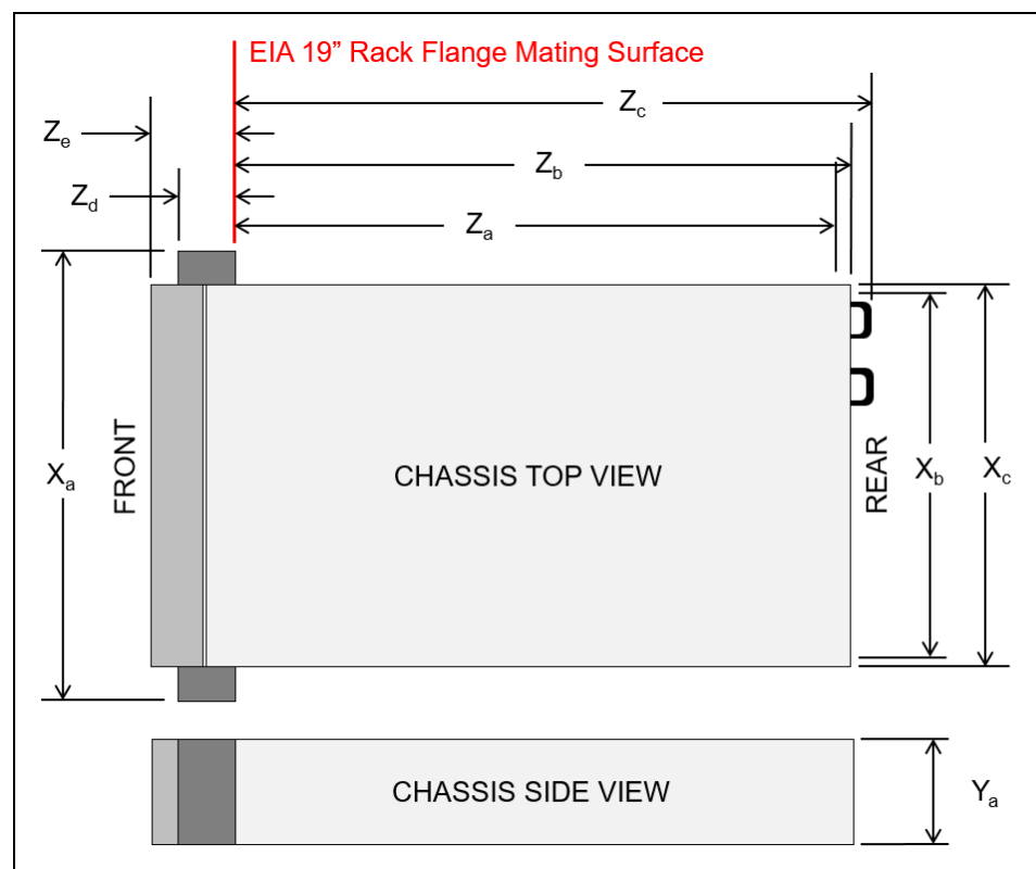
Figure 28. Server dimensions
