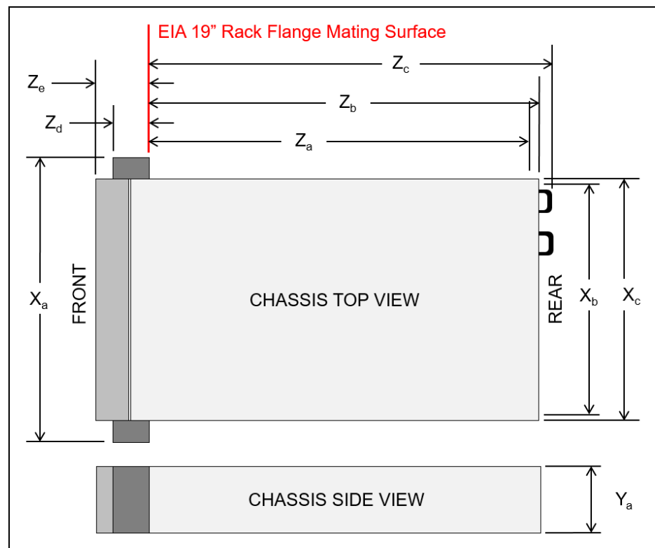
Figure 23. Server dimensions
